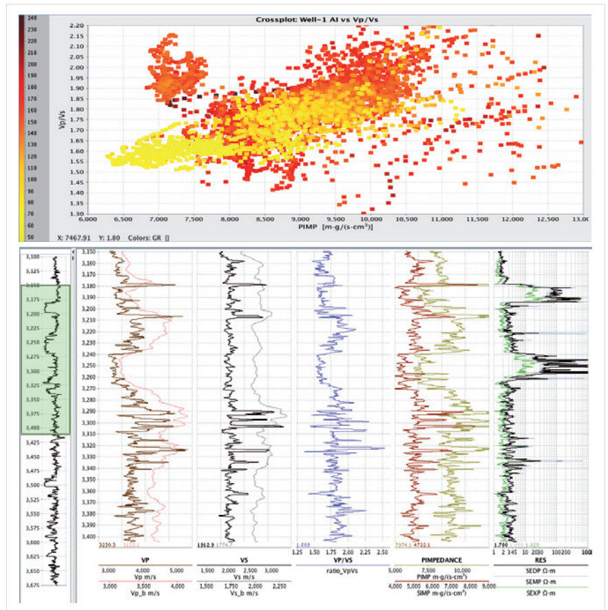
Visualisation of well log data including template functionality and crossplotting.
