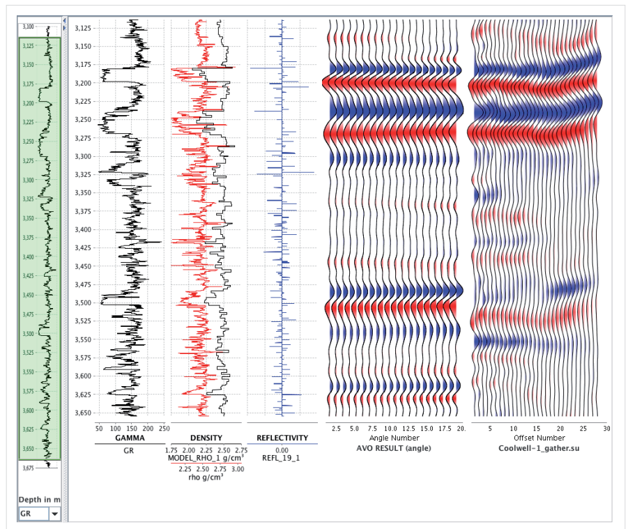
Deterministic AVO modelling of gathers.
