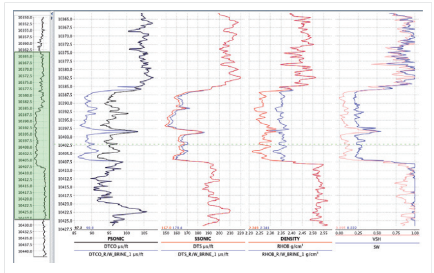
Gassmann fluid substitution with user-defined constraints.
